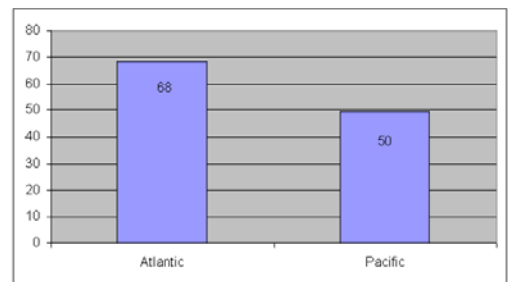
Figure 3. Percentage of events change when QuikSCAT was available.
