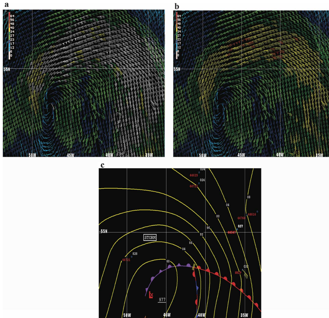
FIG. 9. QuikSCAT winds as in Fig. 7 but (a), (b) at 0800 UTC 4 Nov 2004 centered on 54^{\circ}\text{N} , 43^{\circ}\text{W} . The rain flag is (a) turned on with white wind barbs showing possible rain contamination and (b) turned off. (c) Surface analysis for 0600 UTC 4 Nov 2004 is shown using the convention described in Fig. 7.
