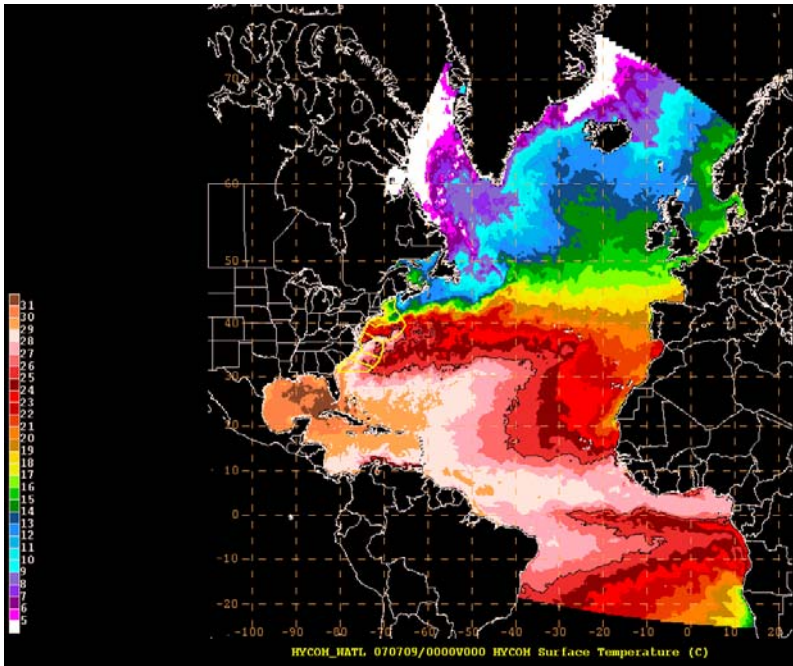
Figure 1. Real Time Ocean Forecast System Atlantic (RT_OFS_ATL) domain as displayed in the operational N-AWIPS workstation.
