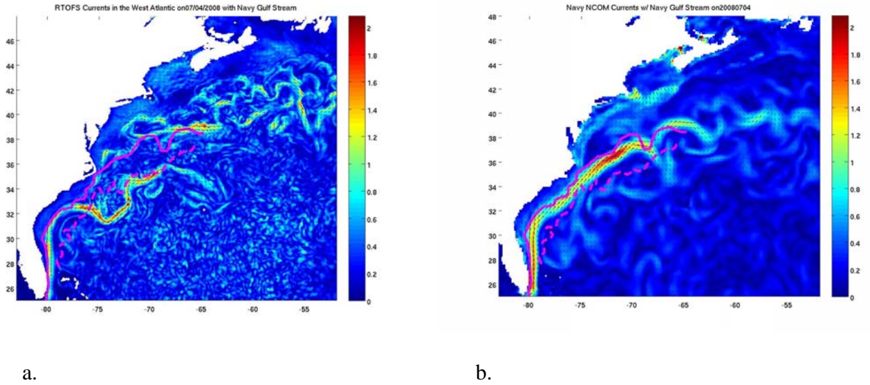
Figure 15. a. RT_OFS Currents with Navy Gulf Stream Analysis in the West Atlantic for July 4, 2008 and b. NCOM Currents with Navy Gulf Stream Analysis in the West Atlantic for July 4, 2008. The Magenta Line is the Navy Gulf Stream Analysis (Solid line = North Wall, Dashed Line = South Wall).
