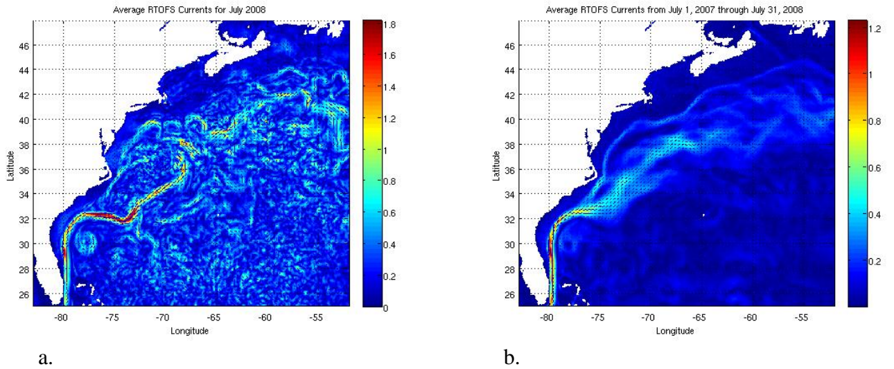
Figure 16. Average of RT_OFS_ATL Currents for a. July 2008 and b. July 1, 2007 through July 31, 2008
